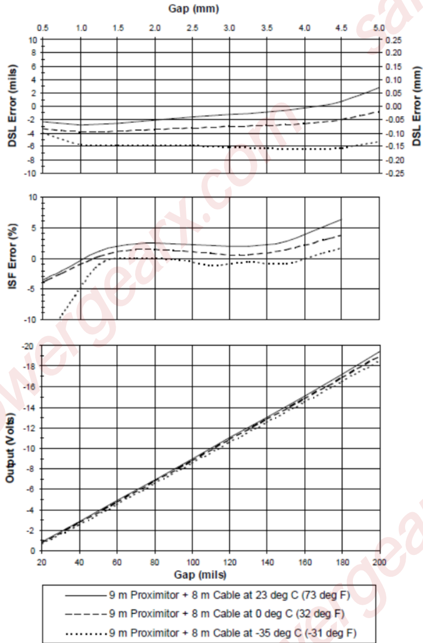
Figure 7: Typical 3300 XL 11 mm 9 m Proximitator Sensor with 8 m of Extension Cable @ Low Temperature
