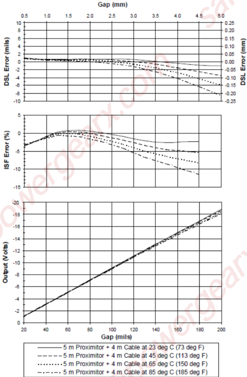
Figure 6: Typical 3300 XL 11 mm 5 m Proximitoer Sensor with 4 m Extension Cable @ High Temperature
