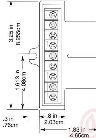
Auxiliary Terminal Block with Barrier Terminals
