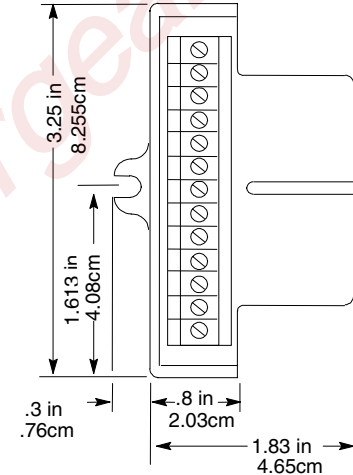
Auxiliary Terminal Block with Box Terminals
