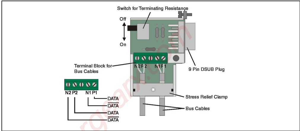
Figure 29: Remote connector
