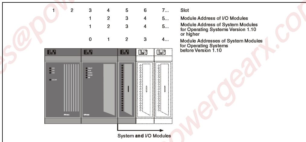
Figure 22: Basic design
