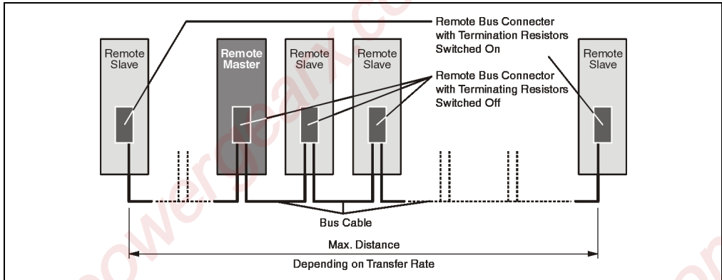
Figure 26: Wiring remote master and slave modules
