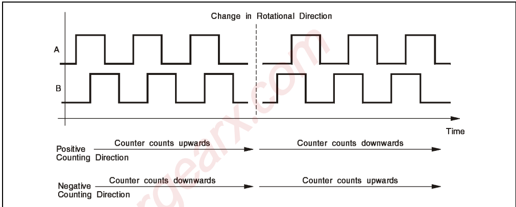
Figure 202: NC150 counting direction in operation mode positioning
