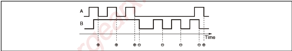
Figure 208: NC150 2 channel, negative edge
