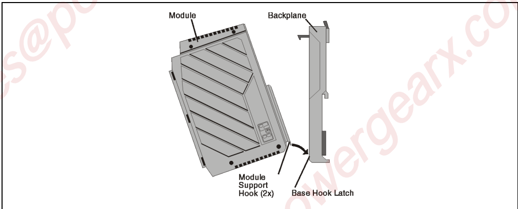
Figure 14: Installing the module
