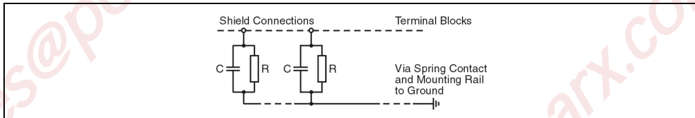
Figure 167: AT660 shielded connection
