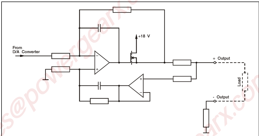
Figure 144: AO775 output circuit diagram
