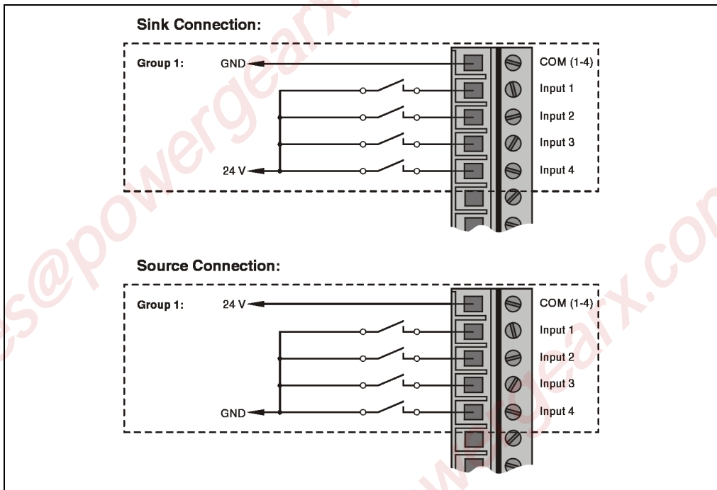
Figure 80: Digital input modules sink/source connections
