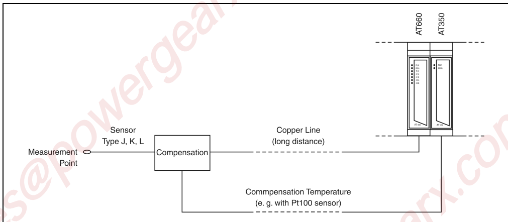
Figure 169: AT660 operation using an external compensation reference junction
