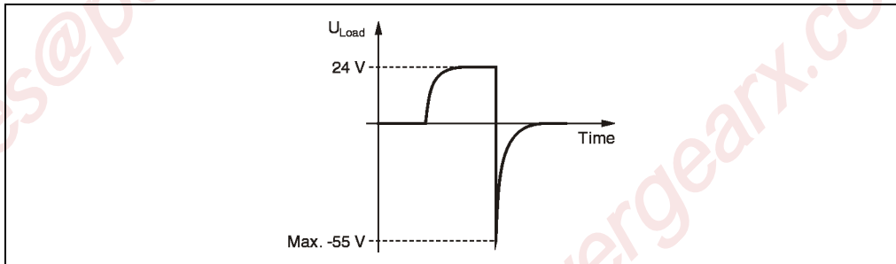
Figure 100: DO479 schematic representation for braking voltage
