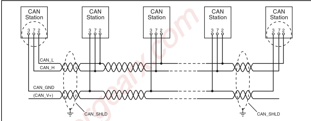
Figure 32: Bus Cable - station connection
