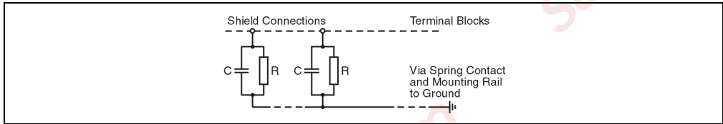
Figure 143: AO775 shielded connection
