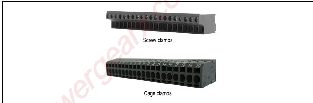
Figure 4: TB170 terminal block
