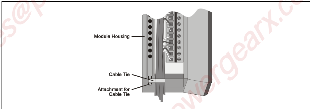
Figure 21: Stress relief using cable ties
