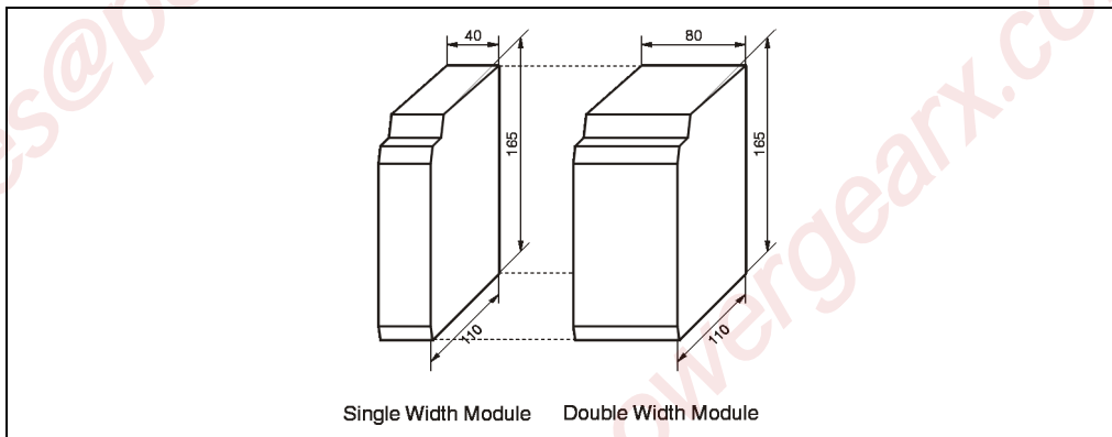
Figure 8: B&R SYSTEM 2005 module dimensions
