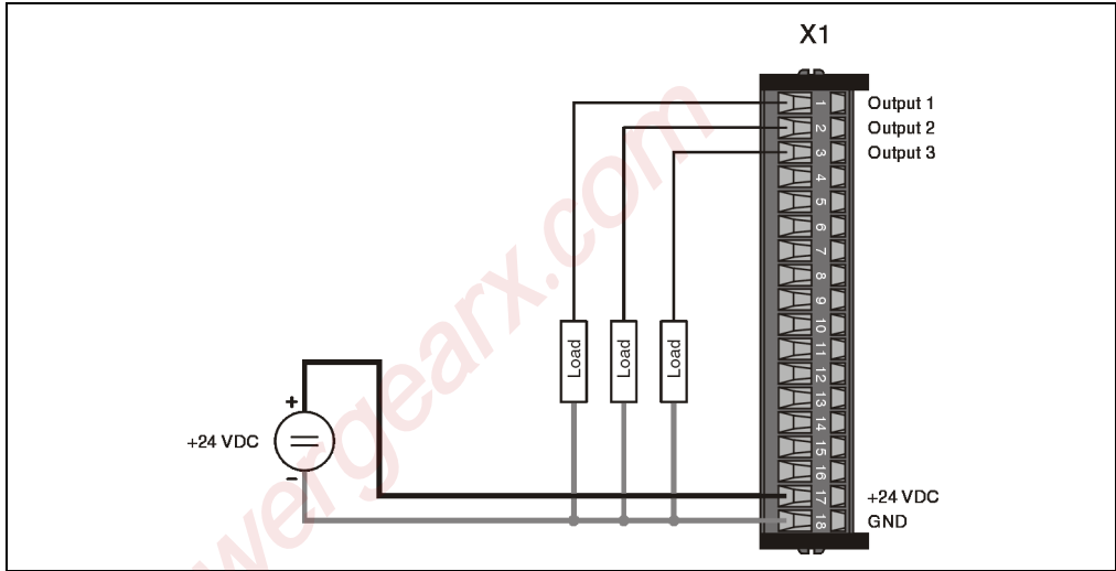
Figure 117: DM486 digital output connection example
