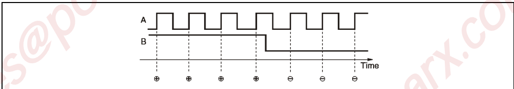
Figure 209: NC150 1 channel, positive edge
