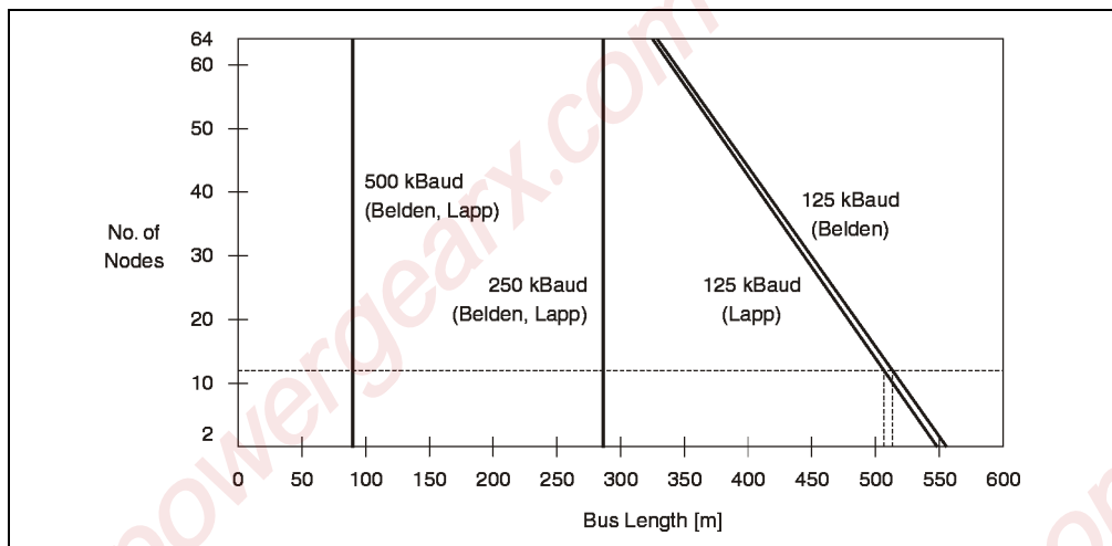
Figure 31: Relationship between the number of nodes and bus length
