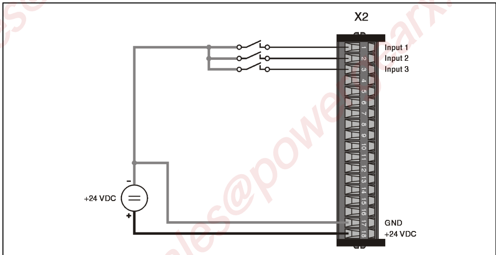
Figure 119: DM486 digital inputs connection examples (source)
