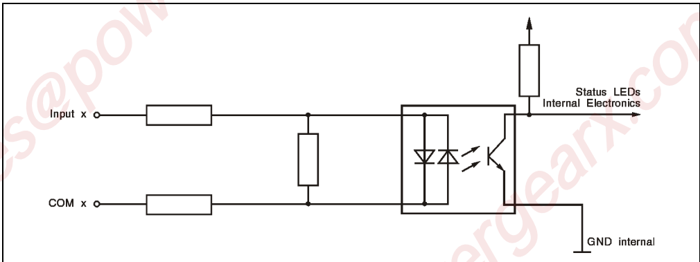
Figure 89: DI450 input circuit diagram for inputs 7 - 16
