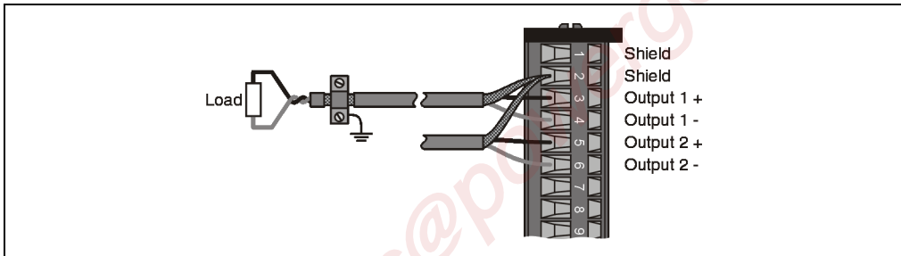
Figure 140: AO360 signal cable connection
