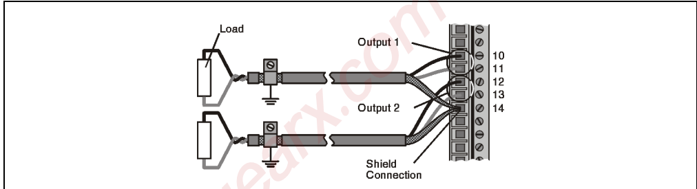
Figure 68: IP161 connection for analog outputs
