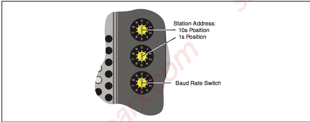
Figure 196: NW150 number switch
