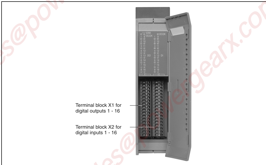
Figure 116: DM486 connection elements
