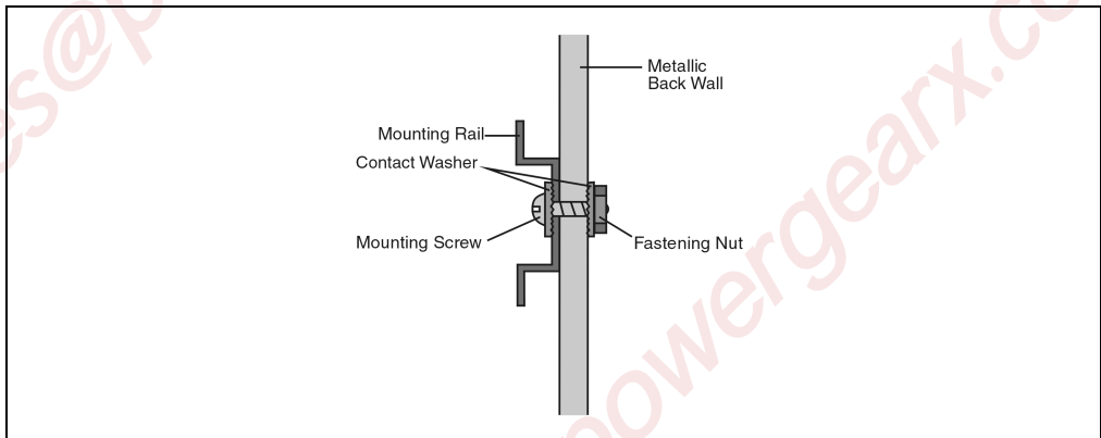
Figure 38: Using a contact washer with lacquered or coated back walls
