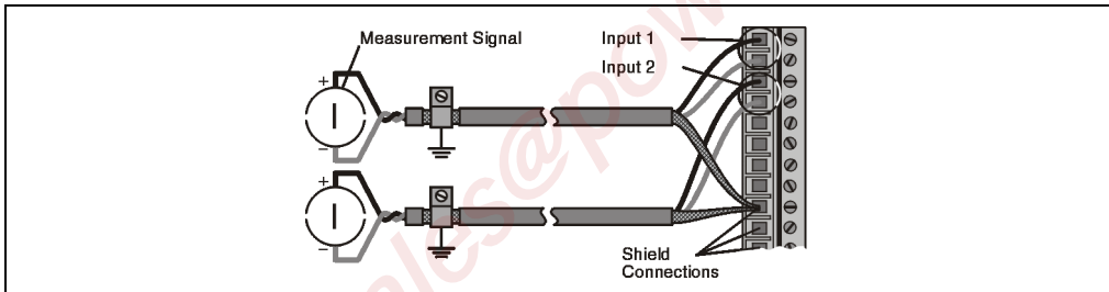
Figure 126: AI775 signal cable connection
