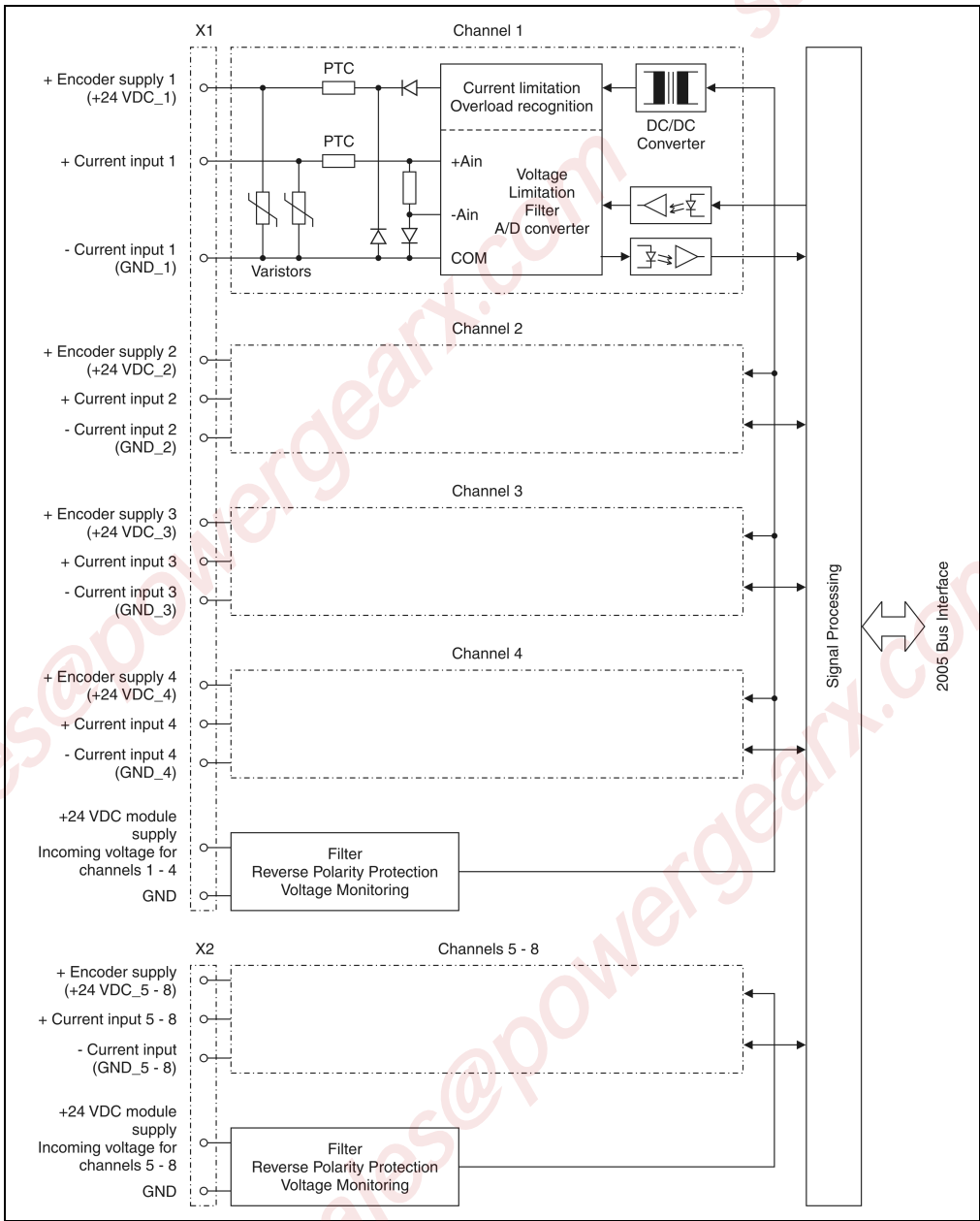
Figure 133: AI780 input circuit diagram
