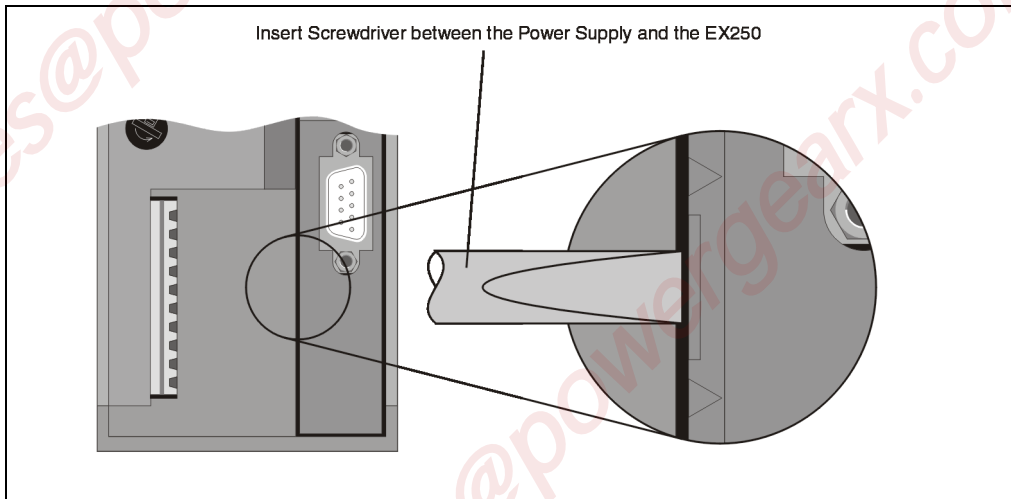
Figure 53: EX250 module fastener
