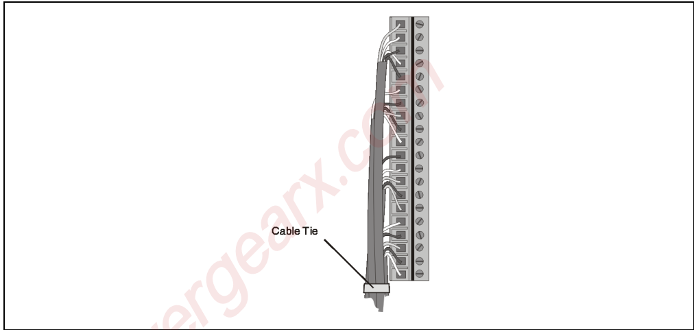
Figure 20: Cabling terminal blocks
