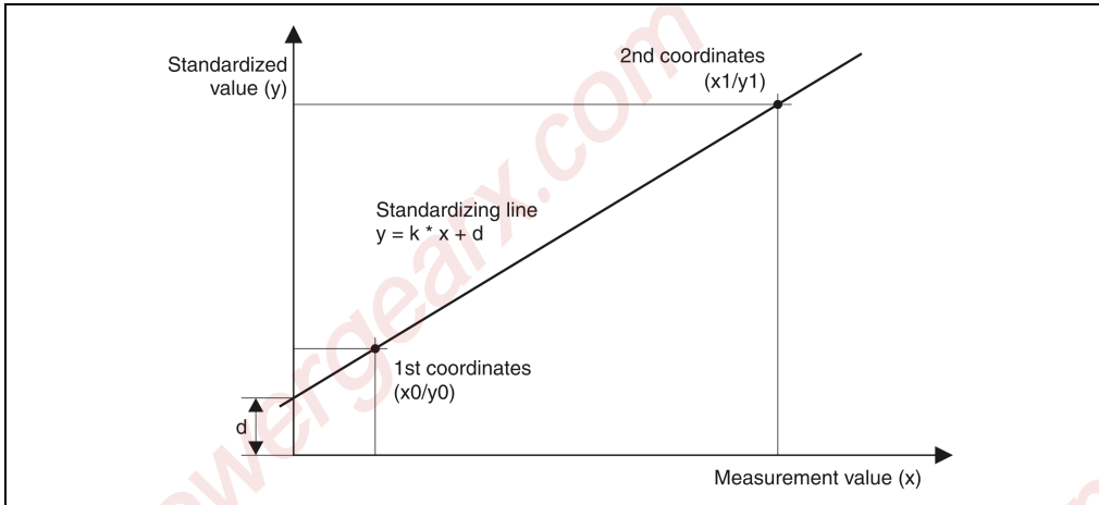
Figure 135: AI780 standardization
