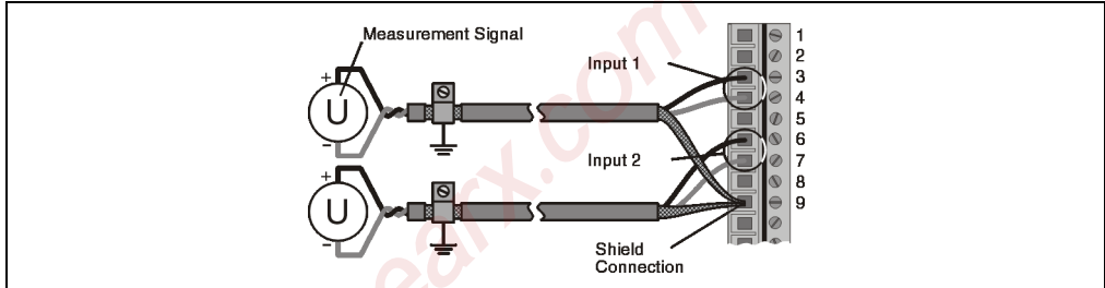
Figure 65: IP161 connections for analog inputs
