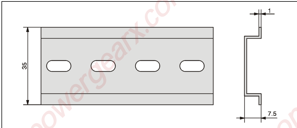
Figure 11: Mounting rail
