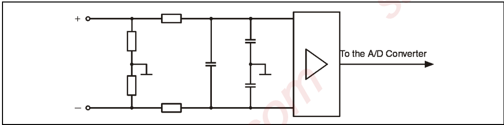
Figure 155: AM055 input circuit diagram
