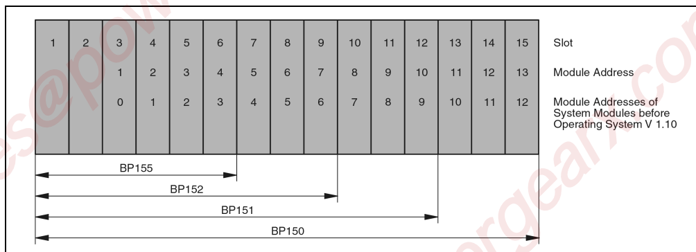
Figure 44: BP15x module address
