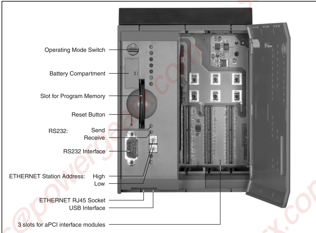
Figure 58: CP382 operational and connection elements
