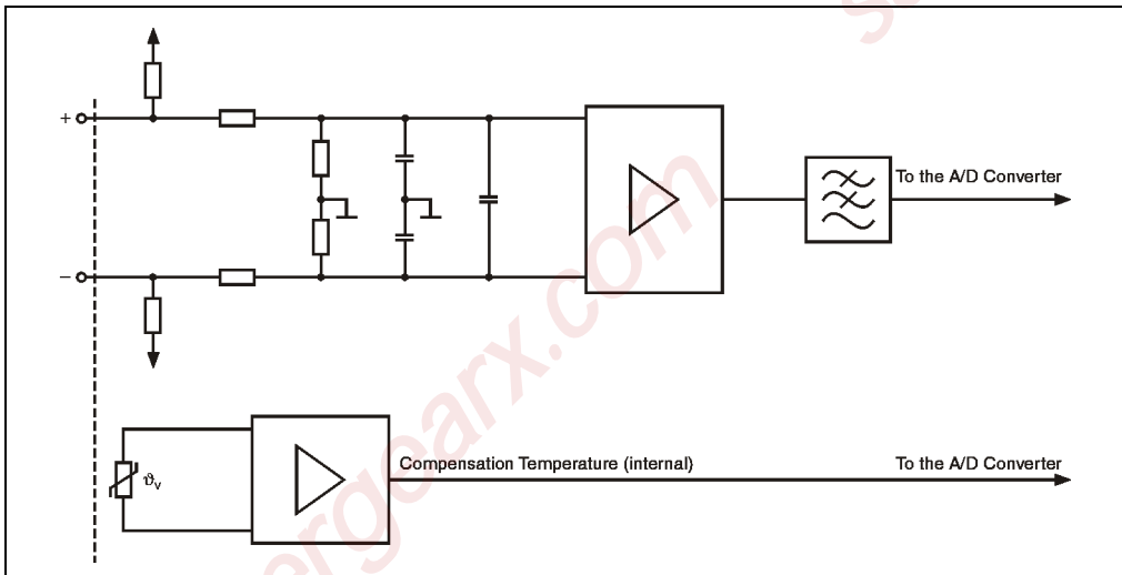
Figure 168: AT660 input circuit diagram
