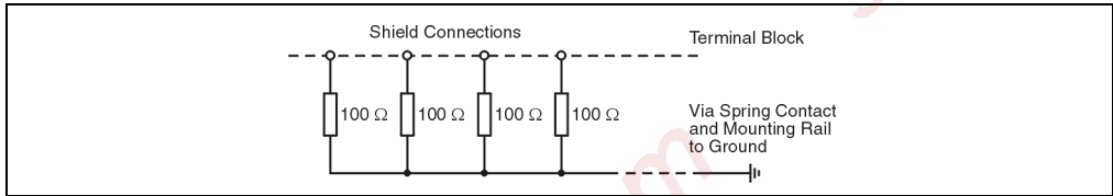
Figure 127: AI775 shielded connection
