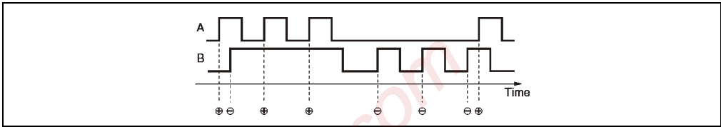
Figure 207: NC150 2 channel, positive edge
