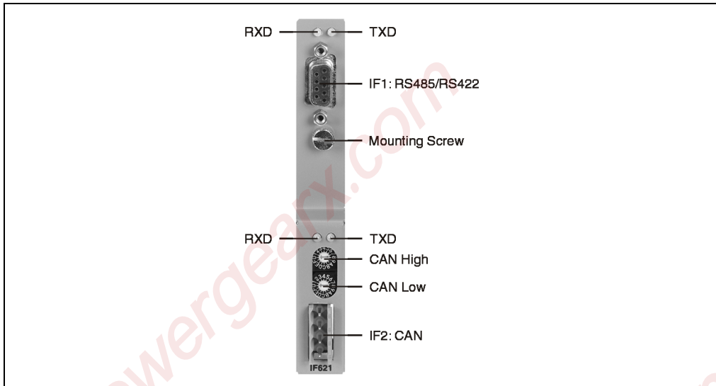
Figure 185: IF621 operational and connection elements
