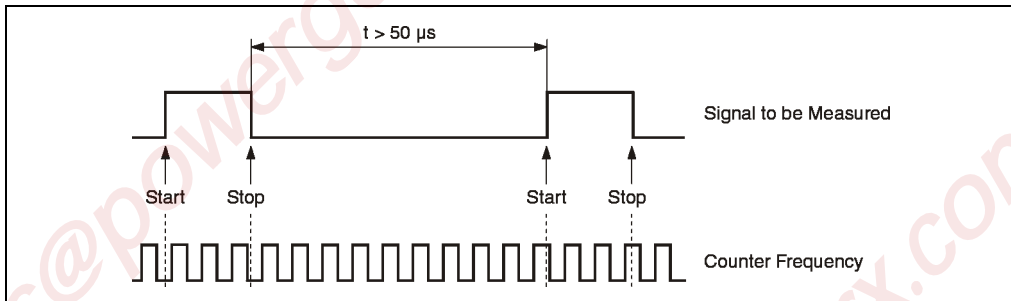
Figure 83: DI450 gate measurement principle
