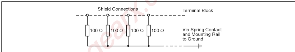
Figure 146: AM050 shielded connection
