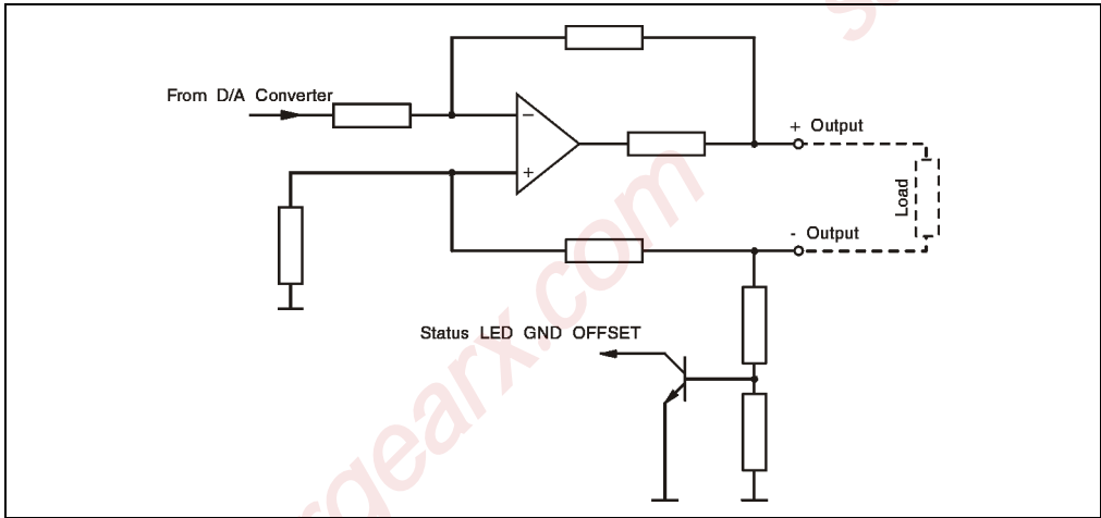
Figure 200: NC150 output diagram for analog outputs
