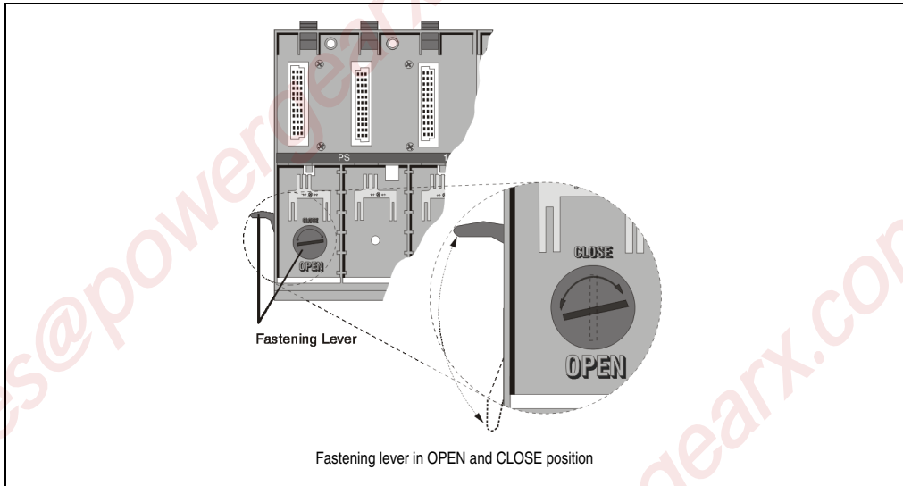
Figure 12: Fastening lever positions
