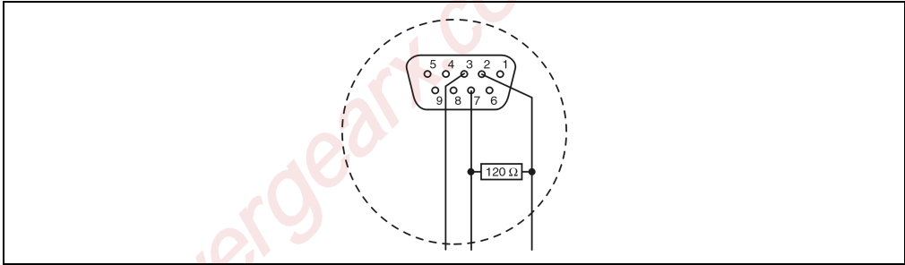
Figure 33: Terminating resistor connections for 9-pin DSUB plug
