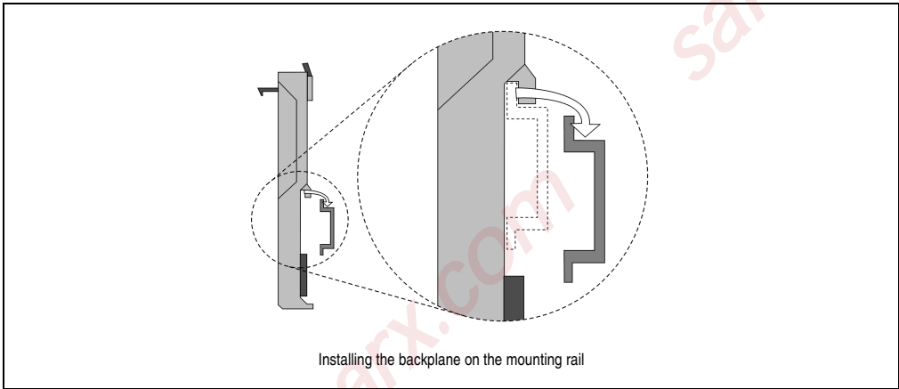
Figure 13: Installing the backplane on the mounting rail
