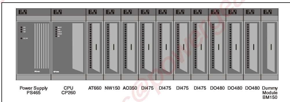
Figure 23: System organization
