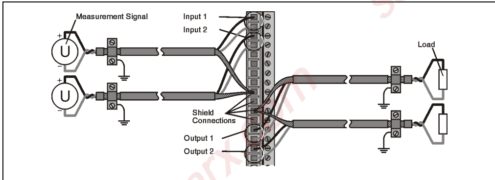
Figure 153: AM055 signal cable connection
