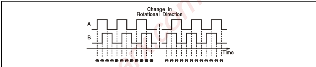
Figure 203: NC150 4x evaluation
