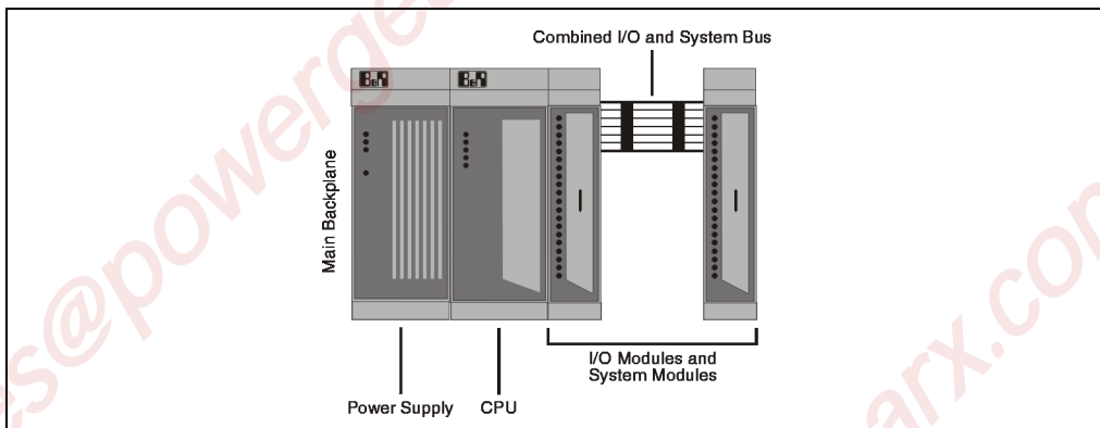
Figure 3: Combined system and I/O bus
