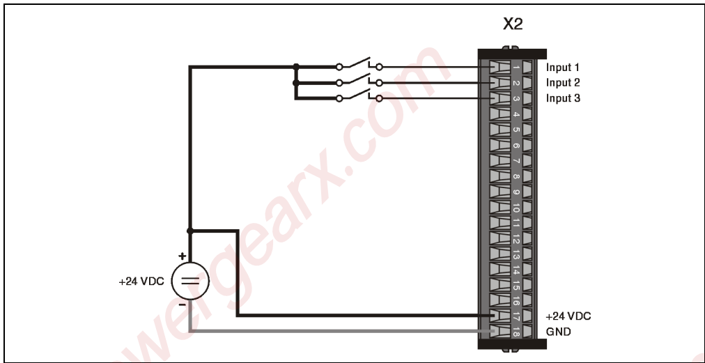
Figure 118: DM486 digital input connection examples (sink)
