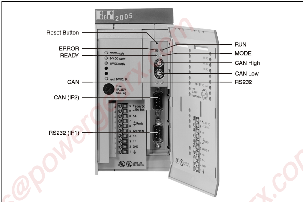
Figure 73: XP152 operational and connection elements
