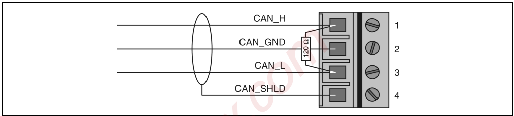
Figure 35: Terminating resistor connections for 4-pin multipoint connector
