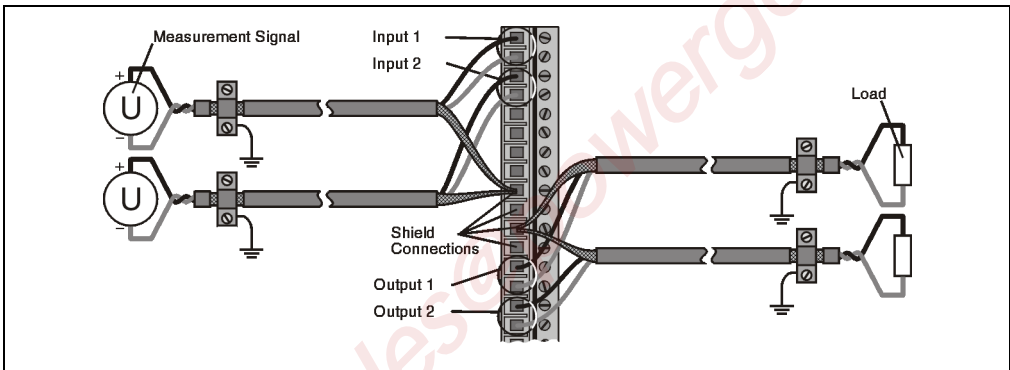
Figure 145: AM050 signal cable connection
