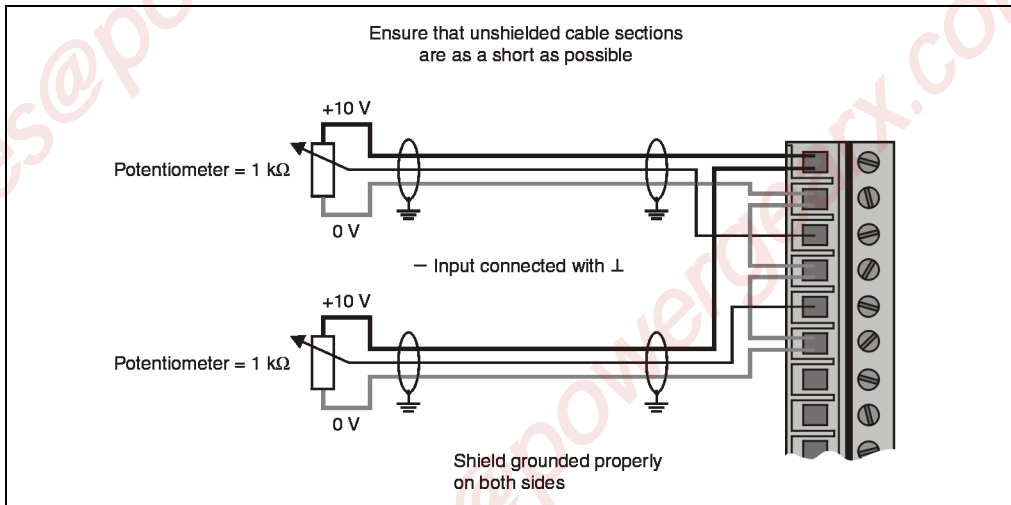
Figure 154: AM055 potentiometer operation
