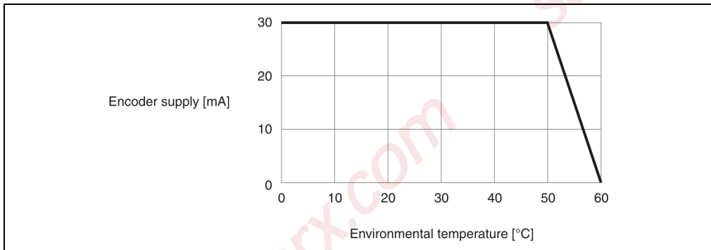
Figure 134: AI780 derating
