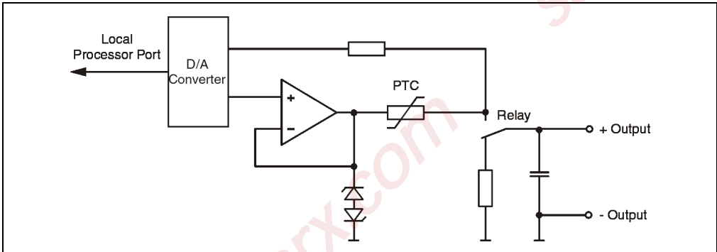
Figure 141: AO360 output circuit diagram
