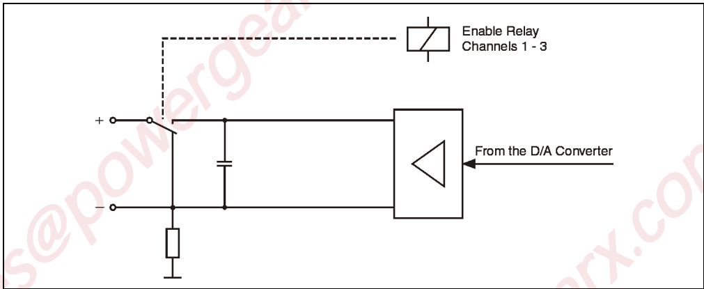
Figure 156: AM055 output circuit diagram
