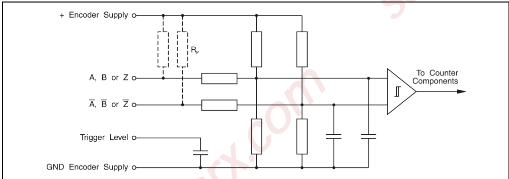
Figure 201: NC150 input circuit for counter inputs
