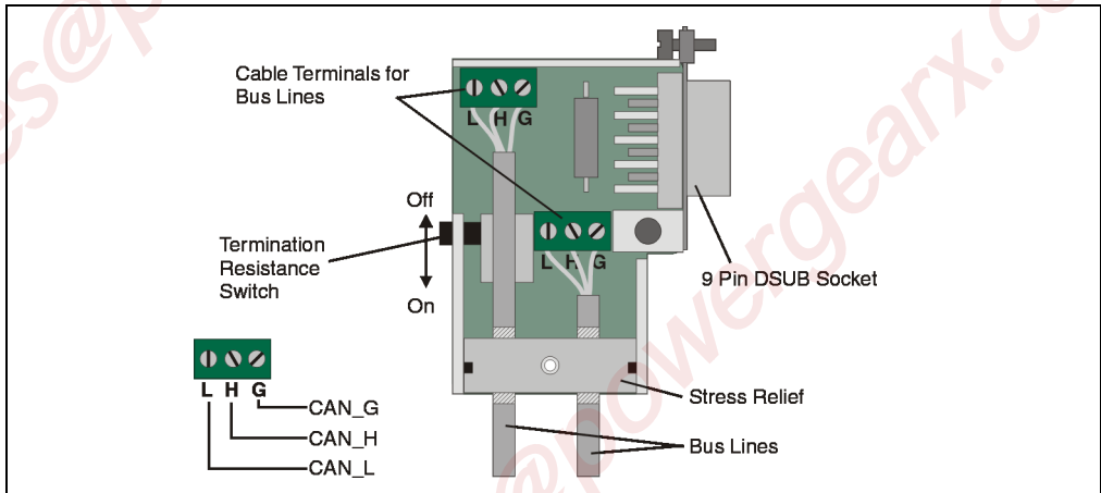
Figure 34: CAN bus connector 7AC911.9
