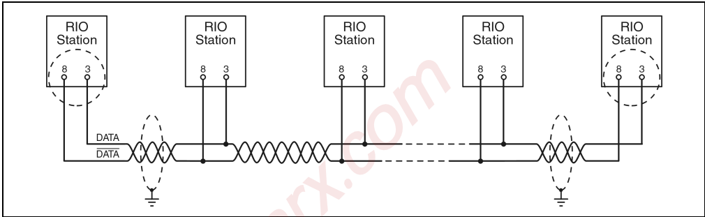
Figure 27: Bus cable ↔ Station connection
