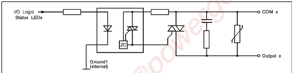
Figure 110: DO690 output circuit diagram
