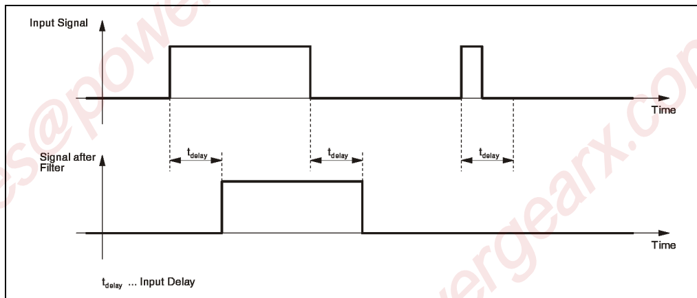
Figure 79: Input filter for digital input modules
