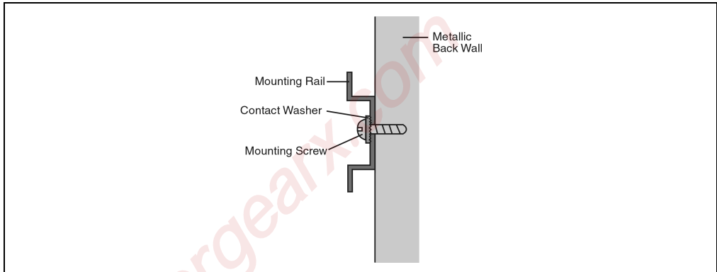
Figure 37: Grounding the mounting rail
