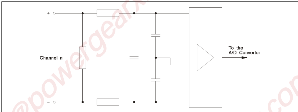
Figure 128: AI775 input circuit diagram
