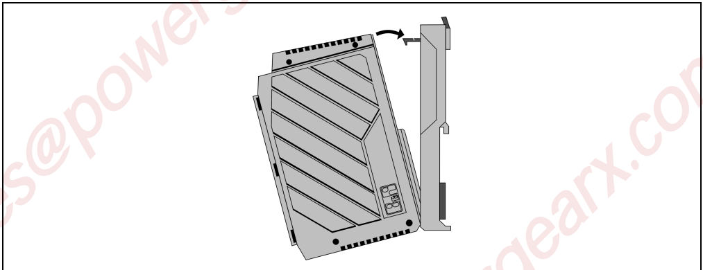
Figure 43: Inserting and removing I/O modules while the controller is running
