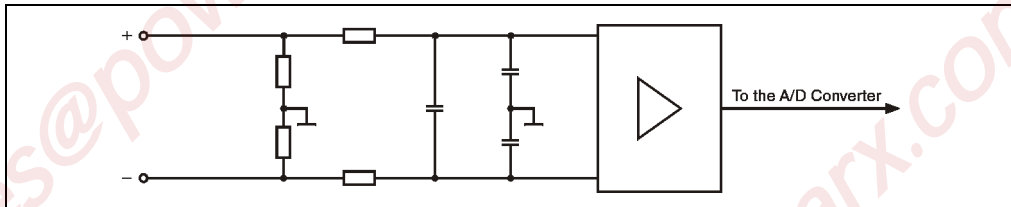
Figure 147: AM050 input circuit diagram
