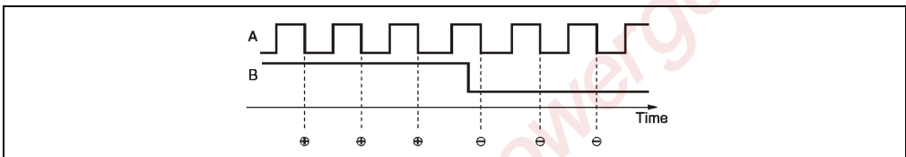
Figure 210: NC150 1 channel, negative edge
