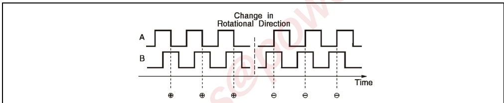
Figure 206: NC150 1x evaluation, negative
