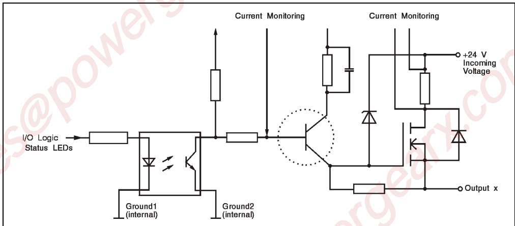
Figure 102: DO480 output circuit diagram
