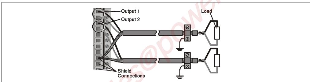
Figure 142: AO775 signal cable connection
