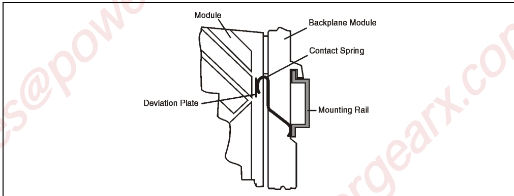
Figure 36: Dissipation of electromagnetic disturbance and grounding via the mounting rail
