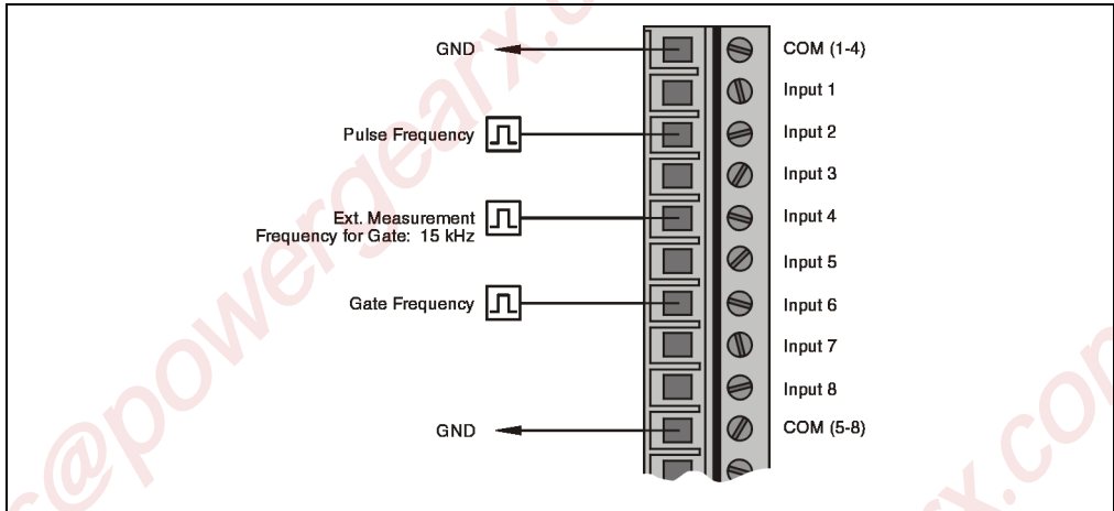
Figure 85: DI450 connection example 2 for gate measurement
