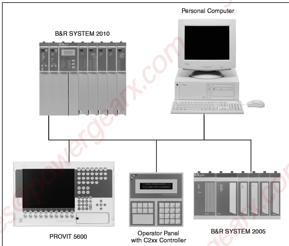
Figure 7: PROFIBUS network
