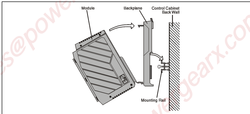
Figure 2: Mounting the B&R SYSTEM 2005 backplane
